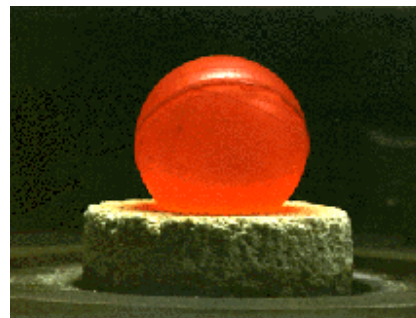
Fusion heat powered red-hot glowing 100 Watt ^{238}\text{PuO}_2 heat source used in the 1970s space missions. The source is about 250 g and about 3 cm in diameter.
